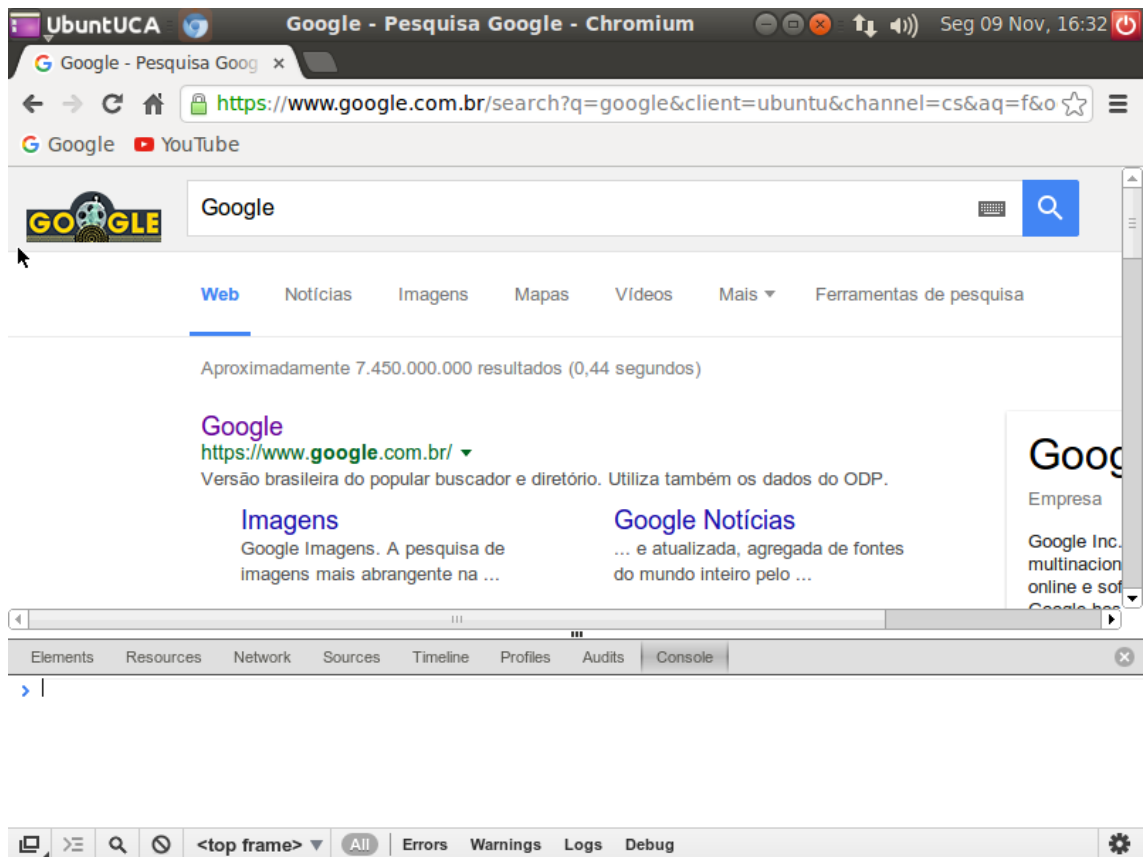
Figura 3.1.21 – Console JavaScript.
