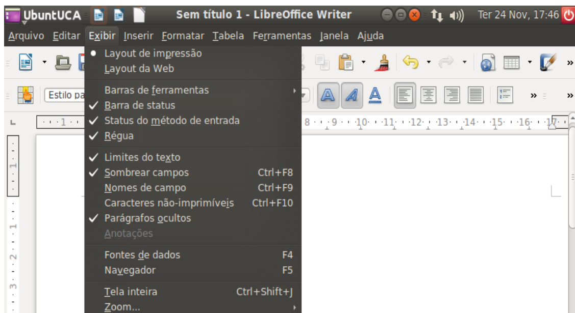
Figura 30: Exibir
