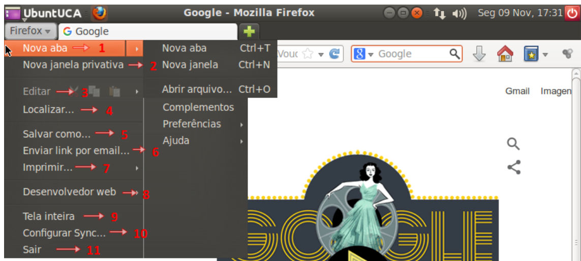
Figura 3.1.2.2 – Firefox.
