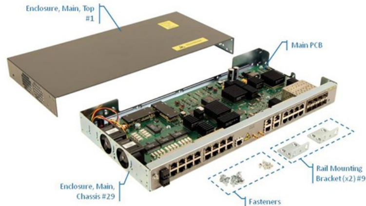
Cisco ASR 901-12C-FT-D Disassembly – Enclosure, Main
